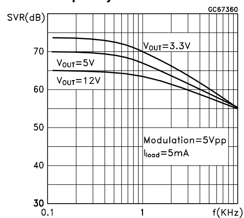
Figure 8. S.V.R. vs Input voltage signal frequency
